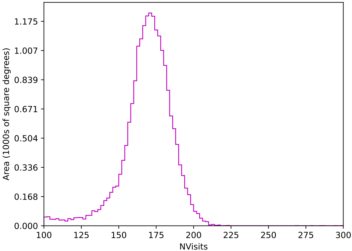
internal_u_expt27_nscale0.9v3.4_10yrs All sky z band: NVisits
