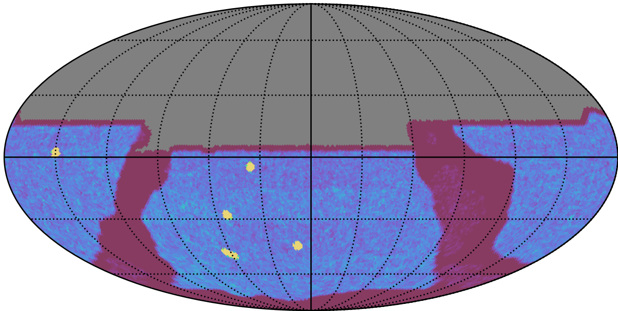
internal_u_expt27_nscale0.9v3.4_10yrs All sky y band: NVisits
