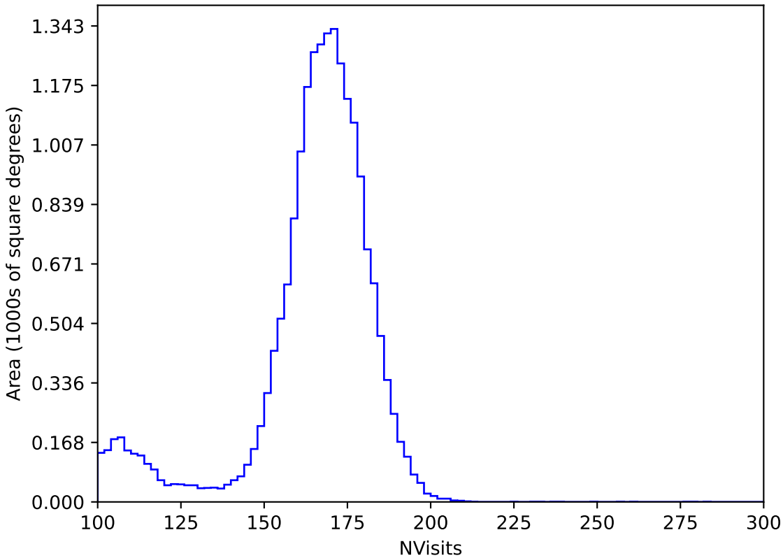
internal_u_expt27_nscale0.9v3.4_10yrs All sky y band: NVisits
