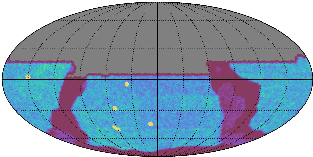
internal_u_expt27_nscale0.9v3.4_10yrs All sky u band: NVisits
