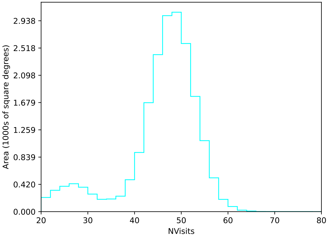
internal_u_expt27_nscale0.9v3.4_10yrs All sky u band: NVisits
