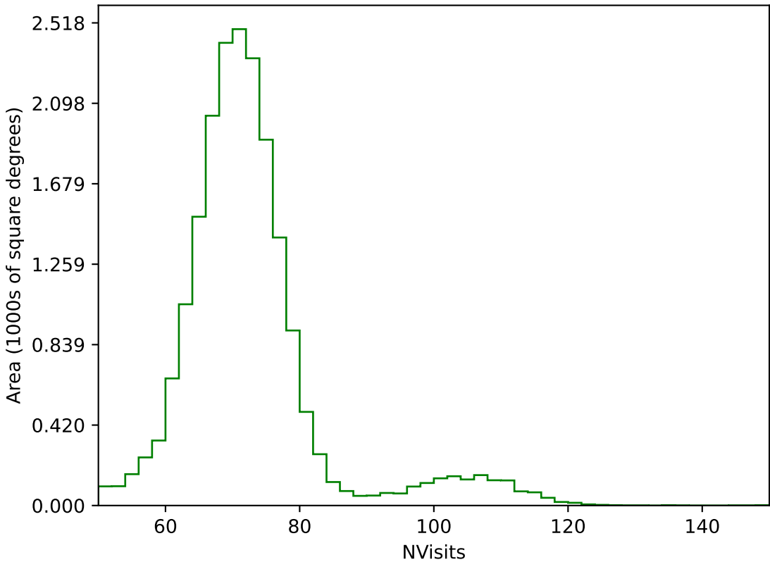
internal_u_expt27_nscale0.9v3.4_10yrs All sky g band: NVisits
