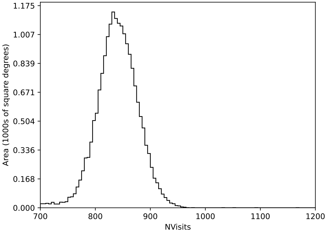
internal_u_expt27_nscale0.9v3.4_10yrs All sky all bands: NVisits
