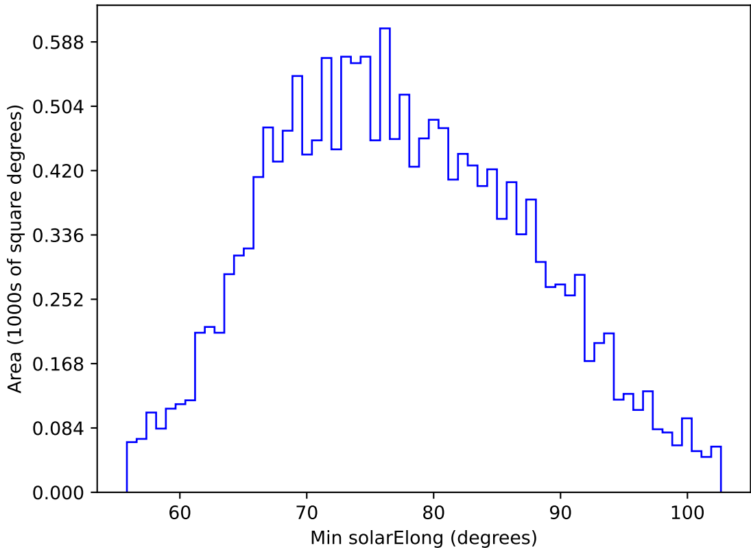
internal_u_expt27_nscale0.9v3.4_10yrs WFD u band: Min solarElong
