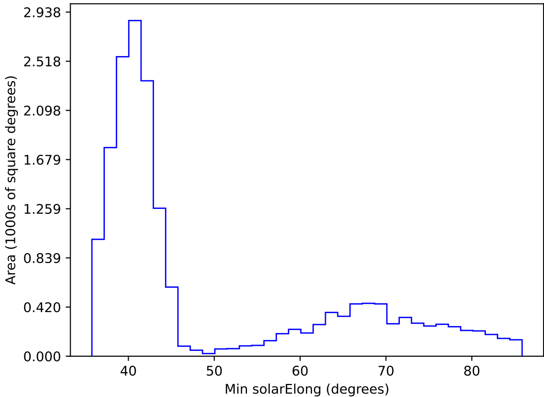
internal_u_expt27_nscale0.9v3.4_10yrs WFD i band: Min solarElong
