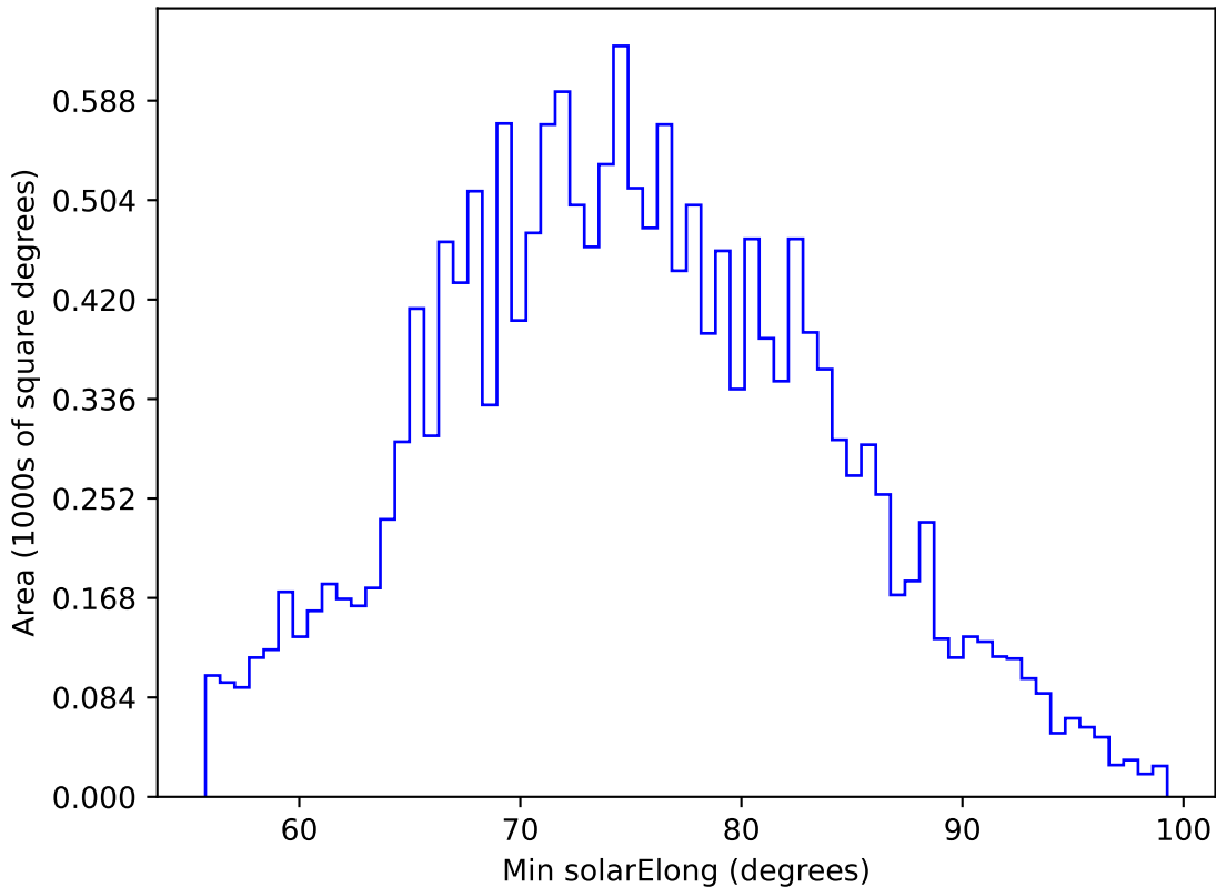
internal_u_expt27_nscale0.9v3.4_10yrs WFD g band: Min solarElong
