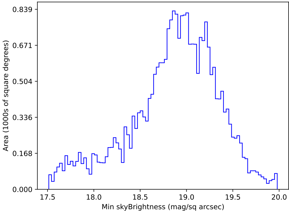
internal_u_expt27_nscale0.9v3.4_10yrs Yr 1 i band: Min skyBrightness
