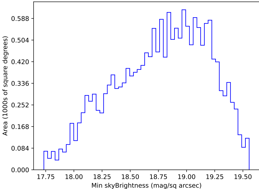
internal_u_expt27_nscale0.9v3.4_10yrs WFD r band: Min skyBrightness
