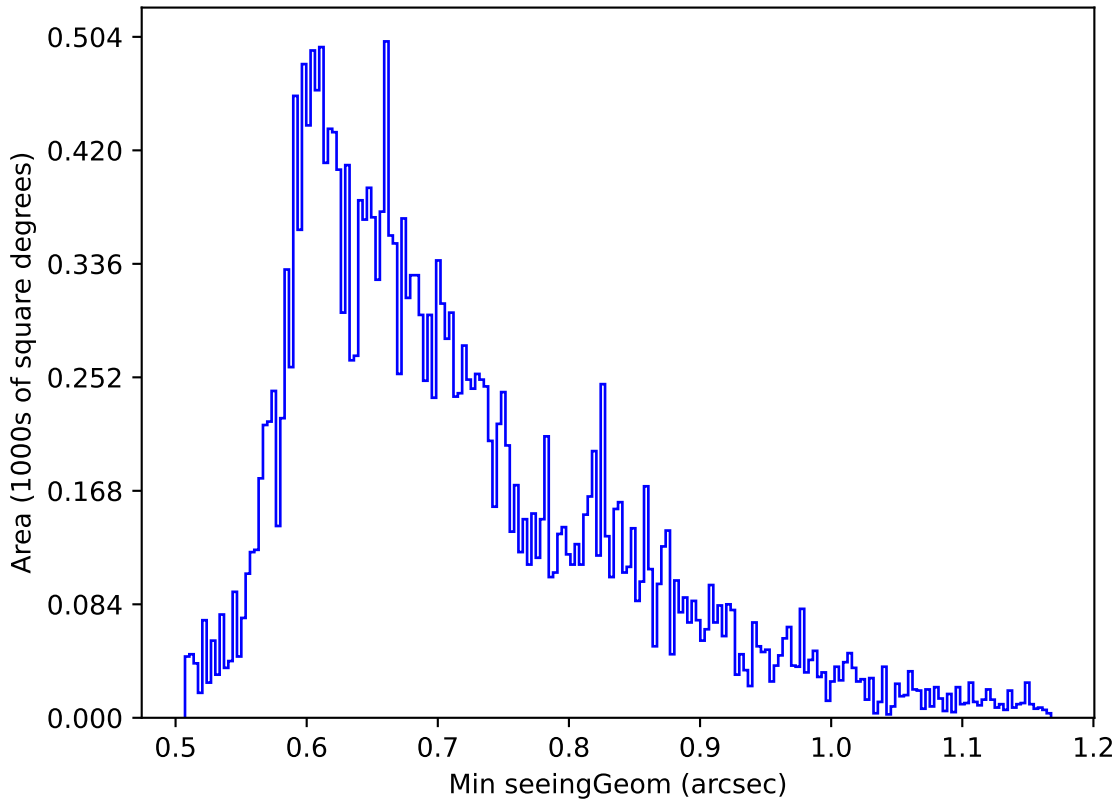
internal_u_expt27_nscale0.9v3.4_10yrs Yr 1 g band: Min seeingGeom
