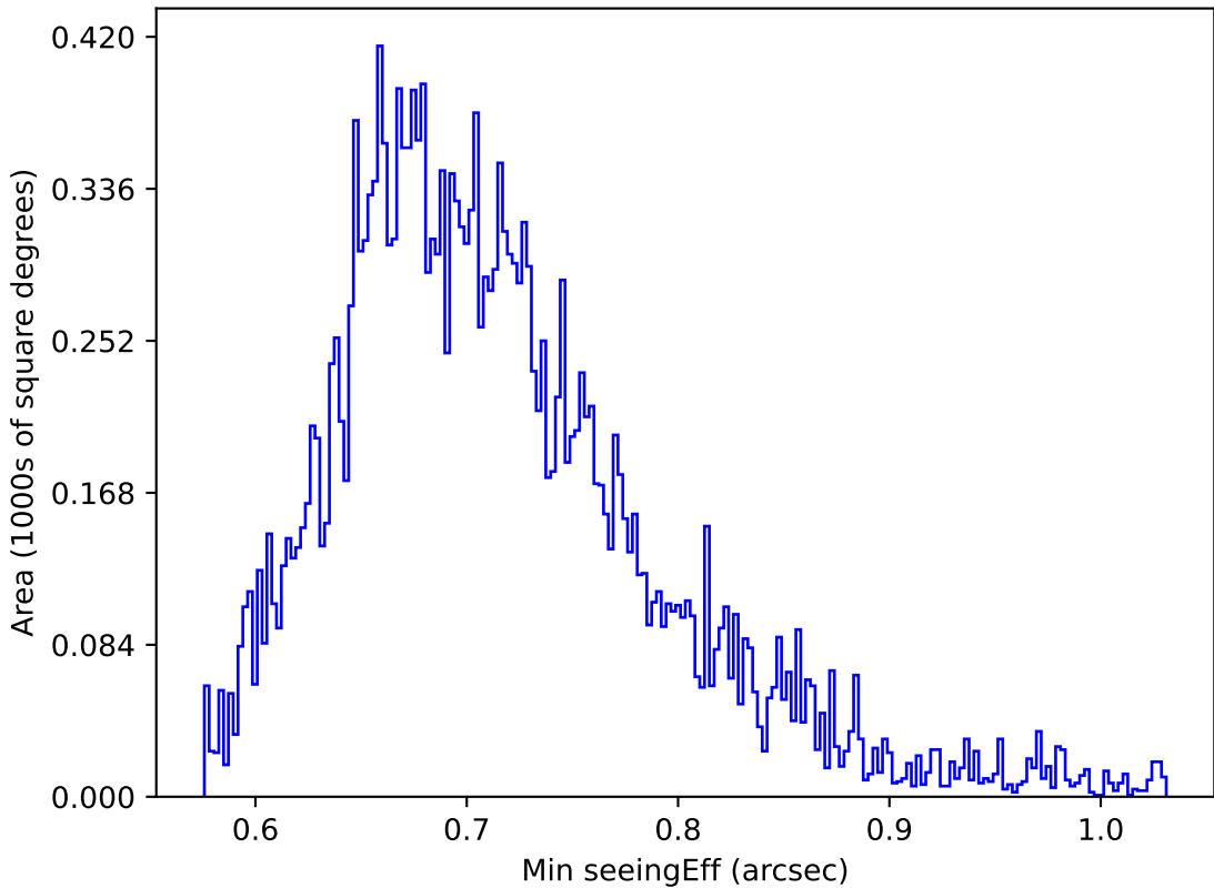
internal_u_expt27_nscale0.9v3.4_10yrs Yr 1 y band: Min seeingEff
