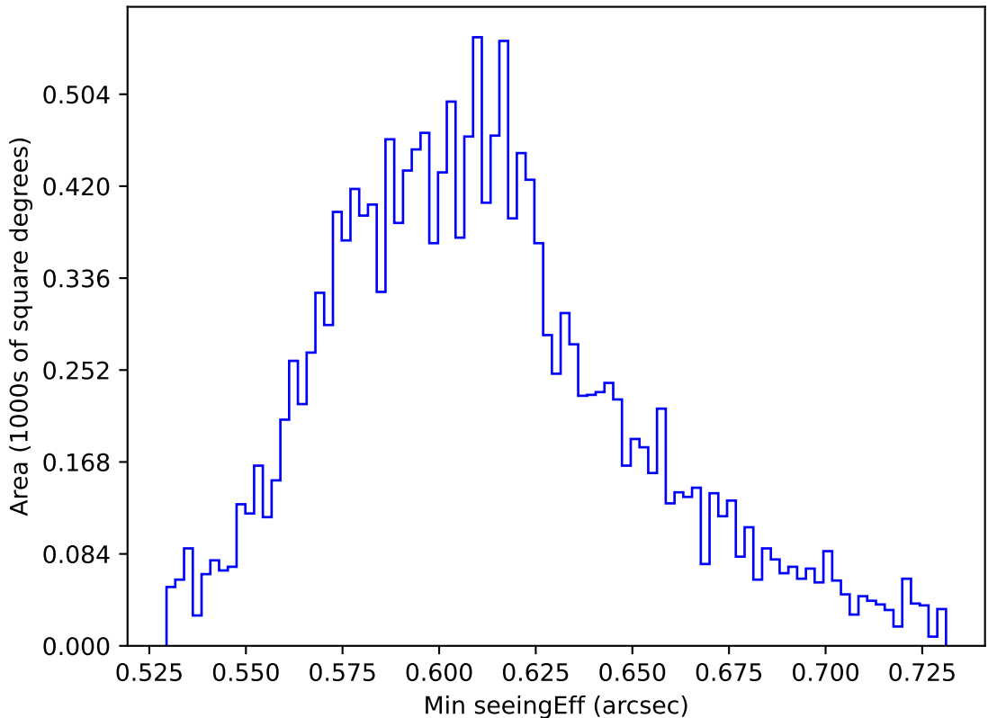
internal_u_expt27_nscale0.9v3.4_10yrs WFD z band: Min seeingEff
