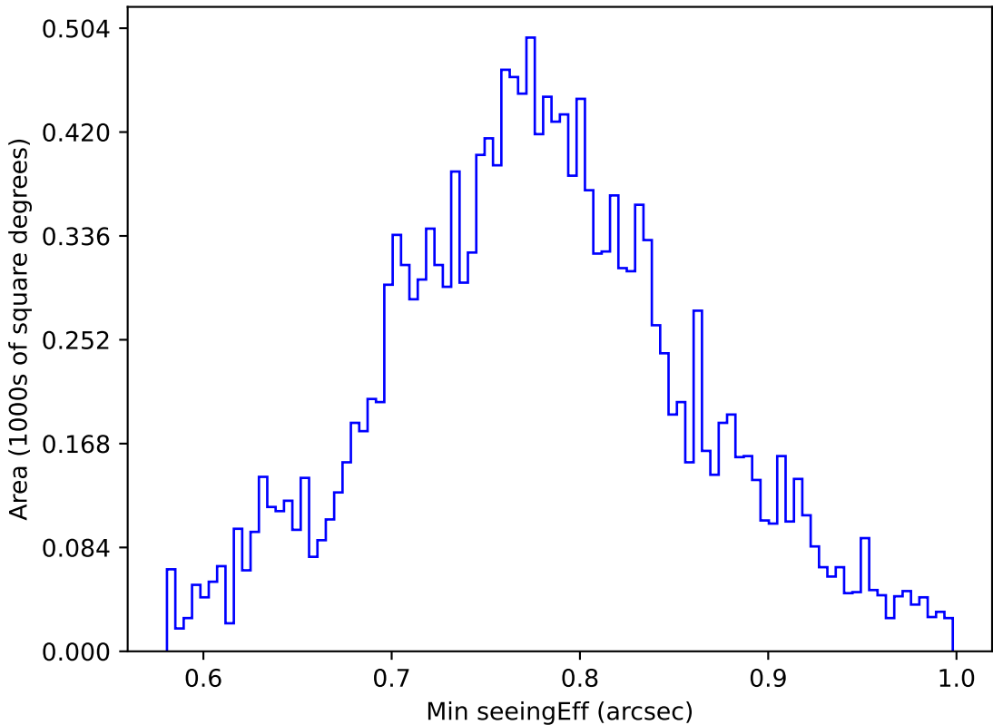
internal_u_expt27_nscale0.9v3.4_10yrs WFD u band: Min seeingEff
