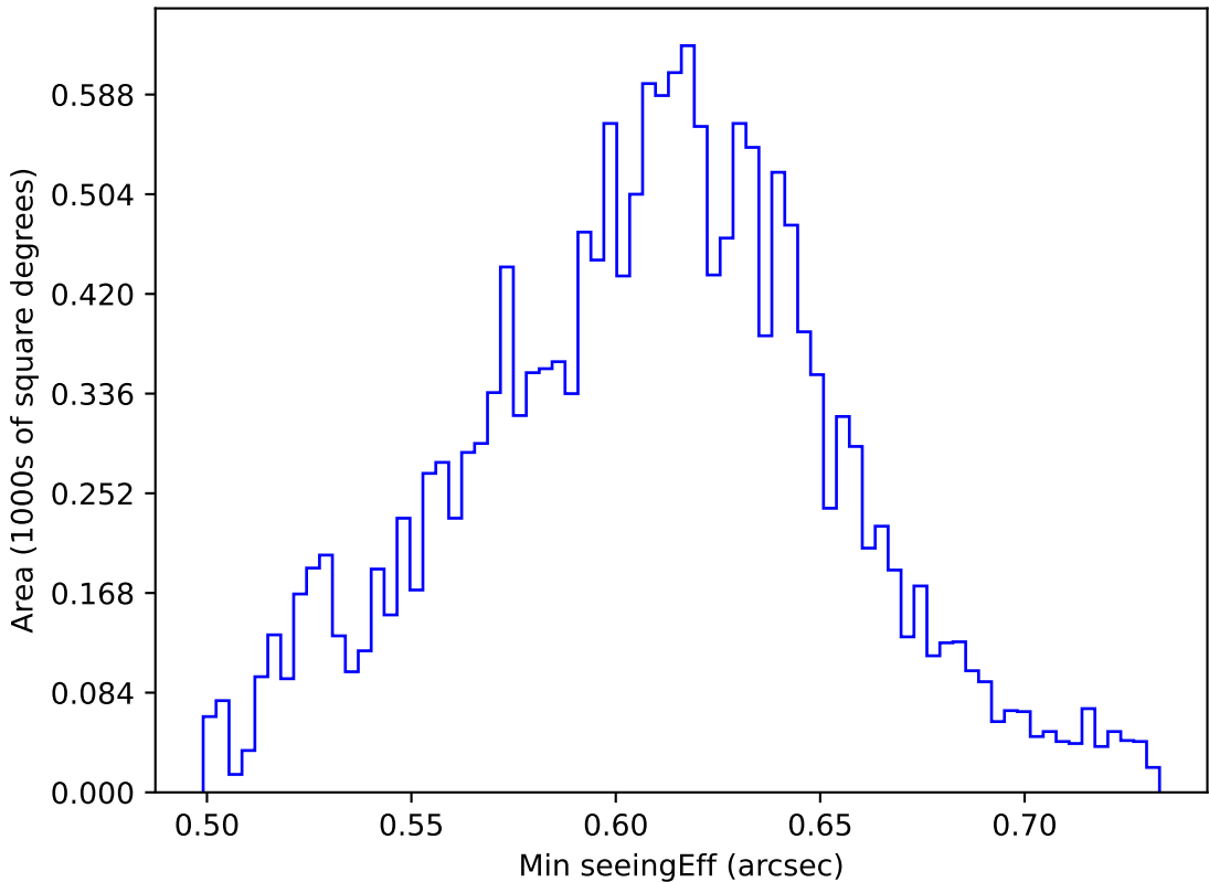
internal_u_expt27_nscale0.9v3.4_10yrs WFD r band: Min seeingEff
