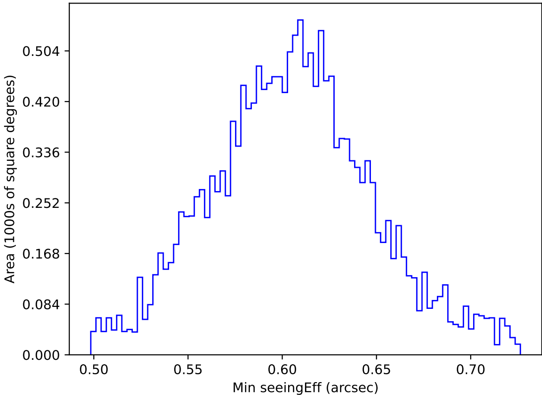
internal_u_expt27_nscale0.9v3.4_10yrs WFD i band: Min seeingEff
