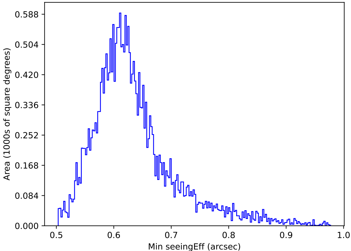
internal_u_expt27_nscale0.9v3.4_10yrs All sky i band: Min seeingEff
