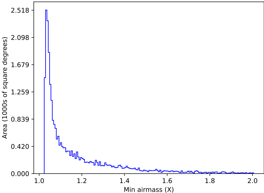
internal_u_expt27_nscale0.9v3.4_10yrs Yr 1 z band: Min airmass
