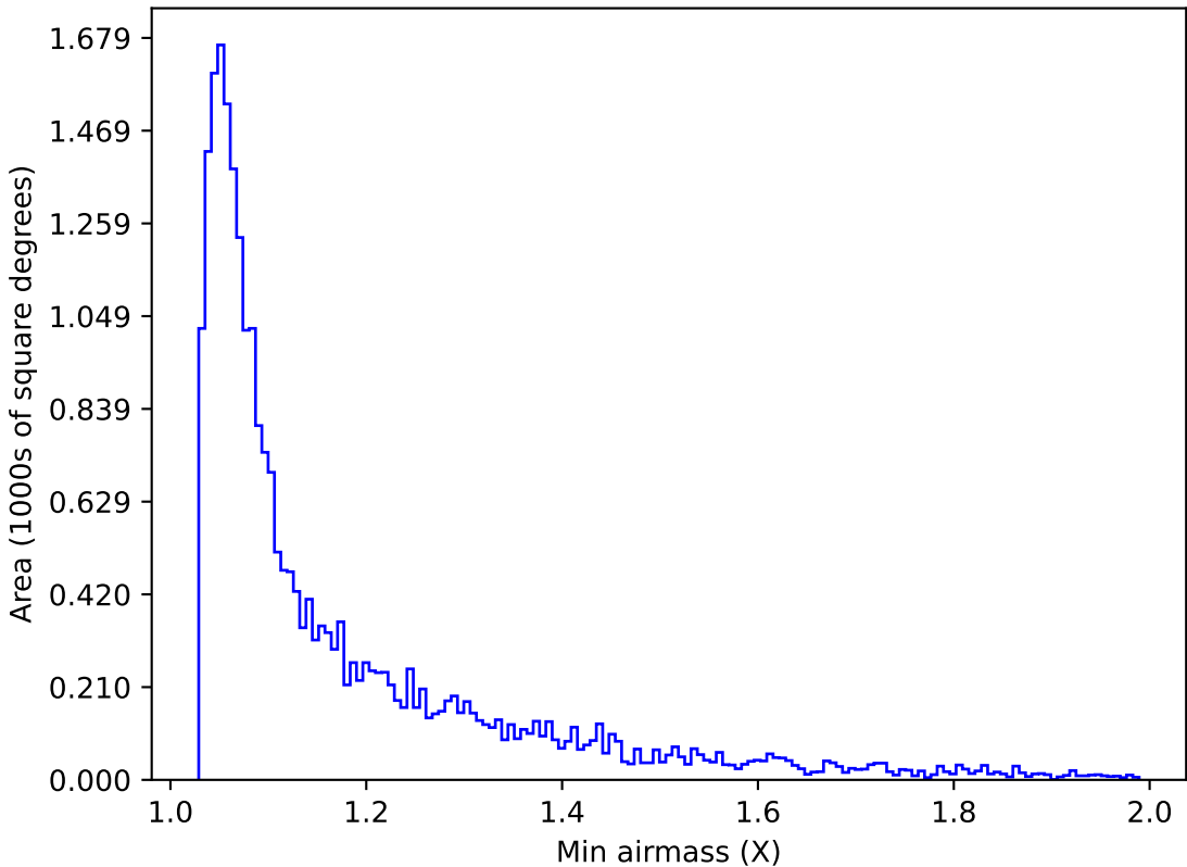
internal_u_expt27_nscale0.9v3.4_10yrs Yr 1 g band: Min airmass
