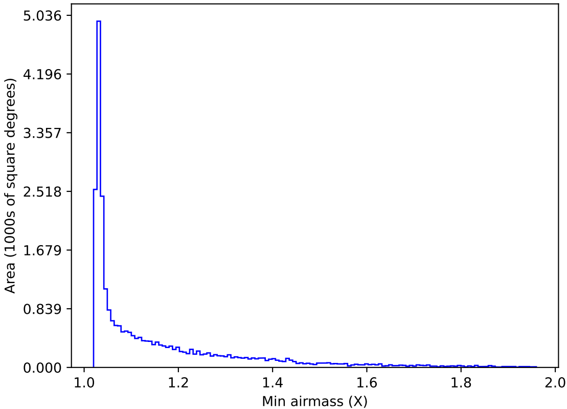
internal_u_expt27_nscale0.9v3.4_10yrs Yr 1 all bands: Min airmass
