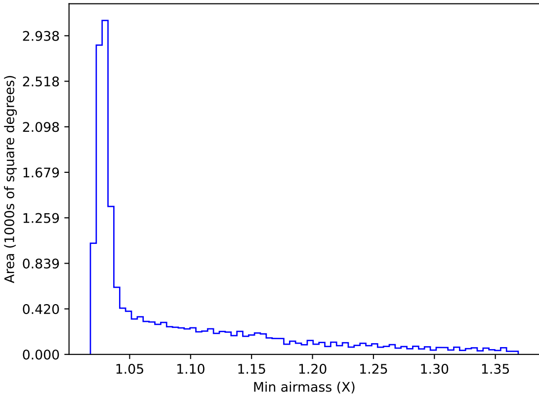
internal_u_expt27_nscale0.9v3.4_10yrs WFD i band: Min airmass
