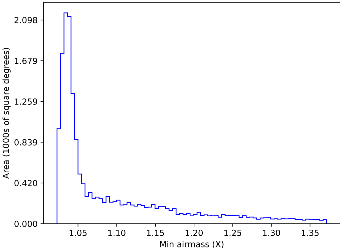
internal_u_expt27_nscale0.9v3.4_10yrs WFD g band: Min airmass
