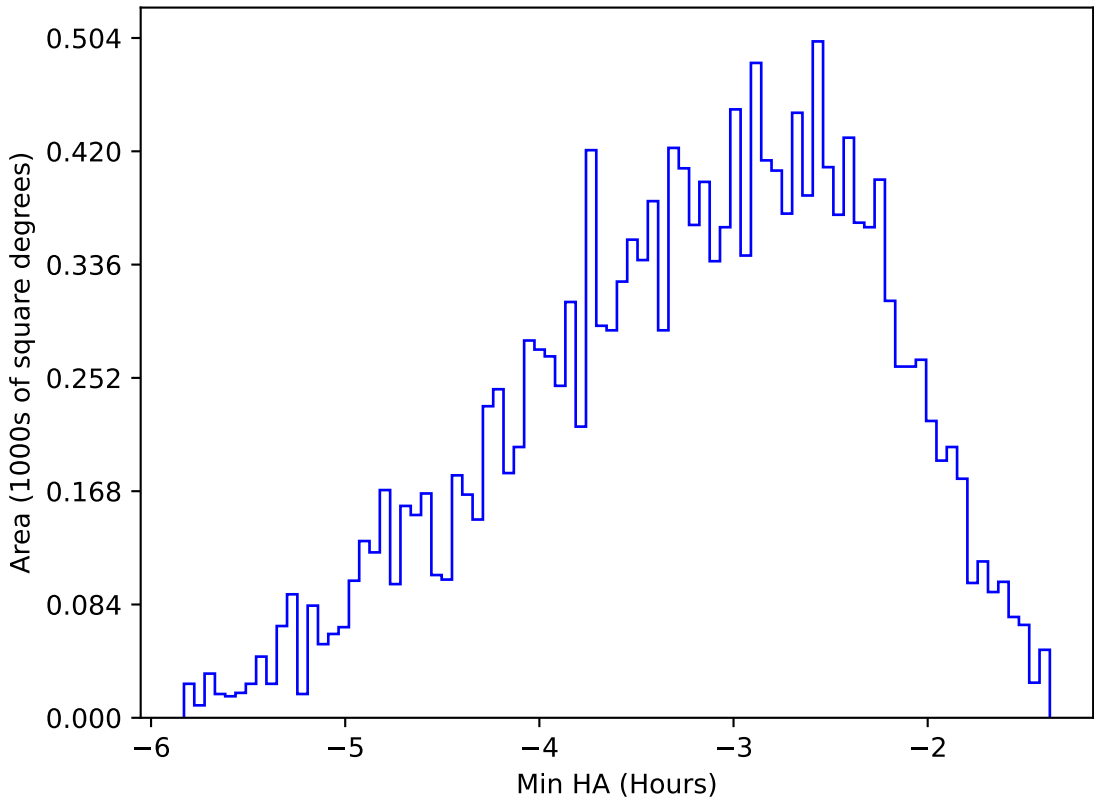
internal_u_expt27_nscale0.9v3.4_10yrs WFD u band: Min HA
