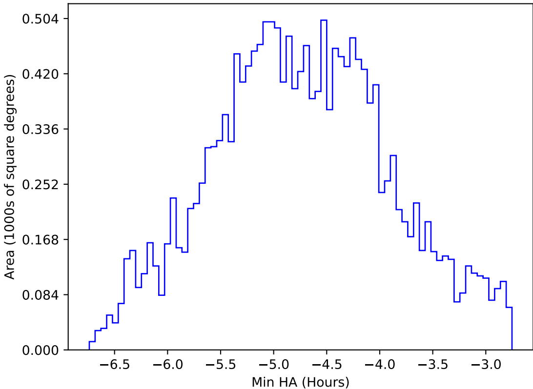
internal_u_expt27_nscale0.9v3.4_10yrs WFD all bands: Min HA
