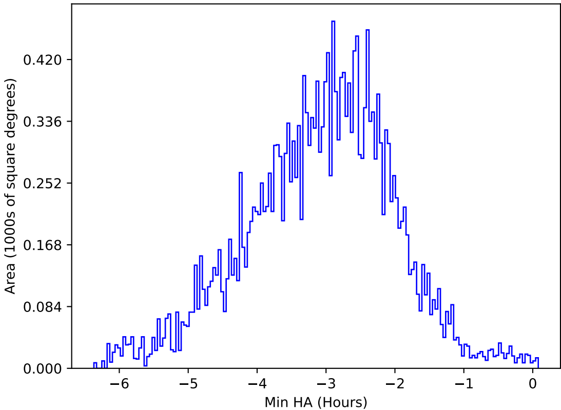
internal_u_expt27_nscale0.9v3.4_10yrs All sky u band: Min HA
