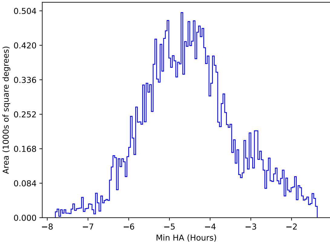
internal_u_expt27_nscale0.9v3.4_10yrs All sky all bands: Min HA
