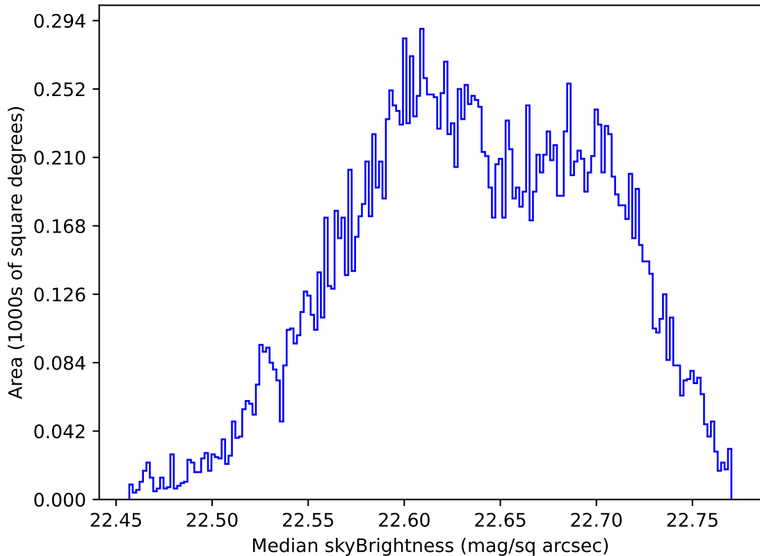
internal_u_expt27_nscale0.9v3.4_10yrs Yr 1 u band: Median skyBrightness
