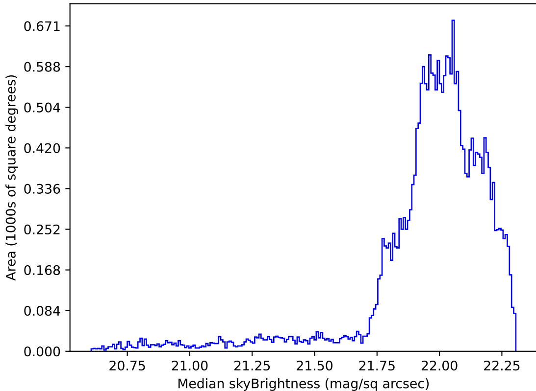
internal_u_expt27_nscale0.9v3.4_10yrs Yr 1 g band: Median skyBrightness
