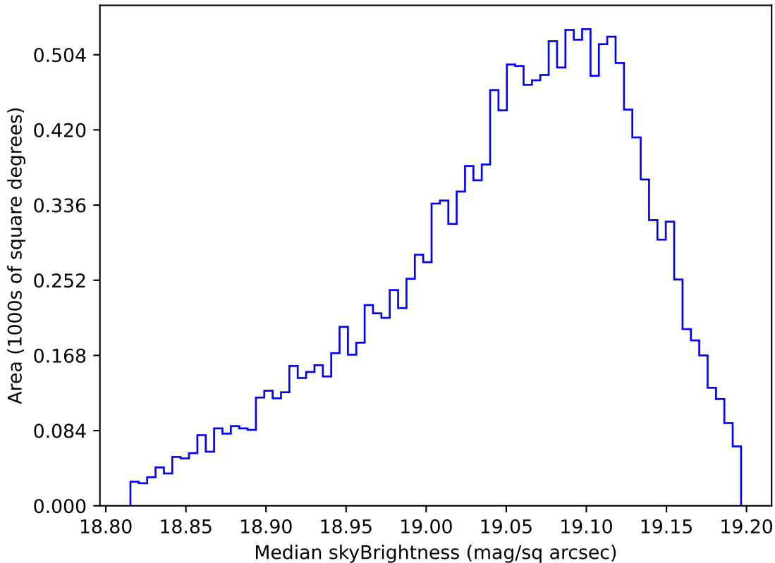
internal_u_expt27_nscale0.9v3.4_10yrs WFD z band: Median skyBrightness
