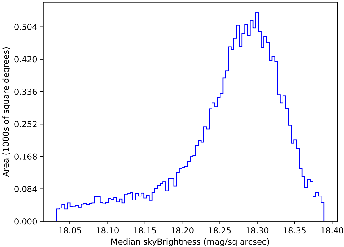
internal_u_expt27_nscale0.9v3.4_10yrs WFD y band: Median skyBrightness
