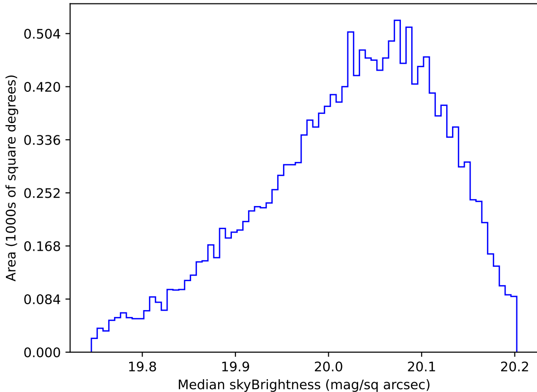
internal_u_expt27_nscale0.9v3.4_10yrs WFD i band: Median skyBrightness
