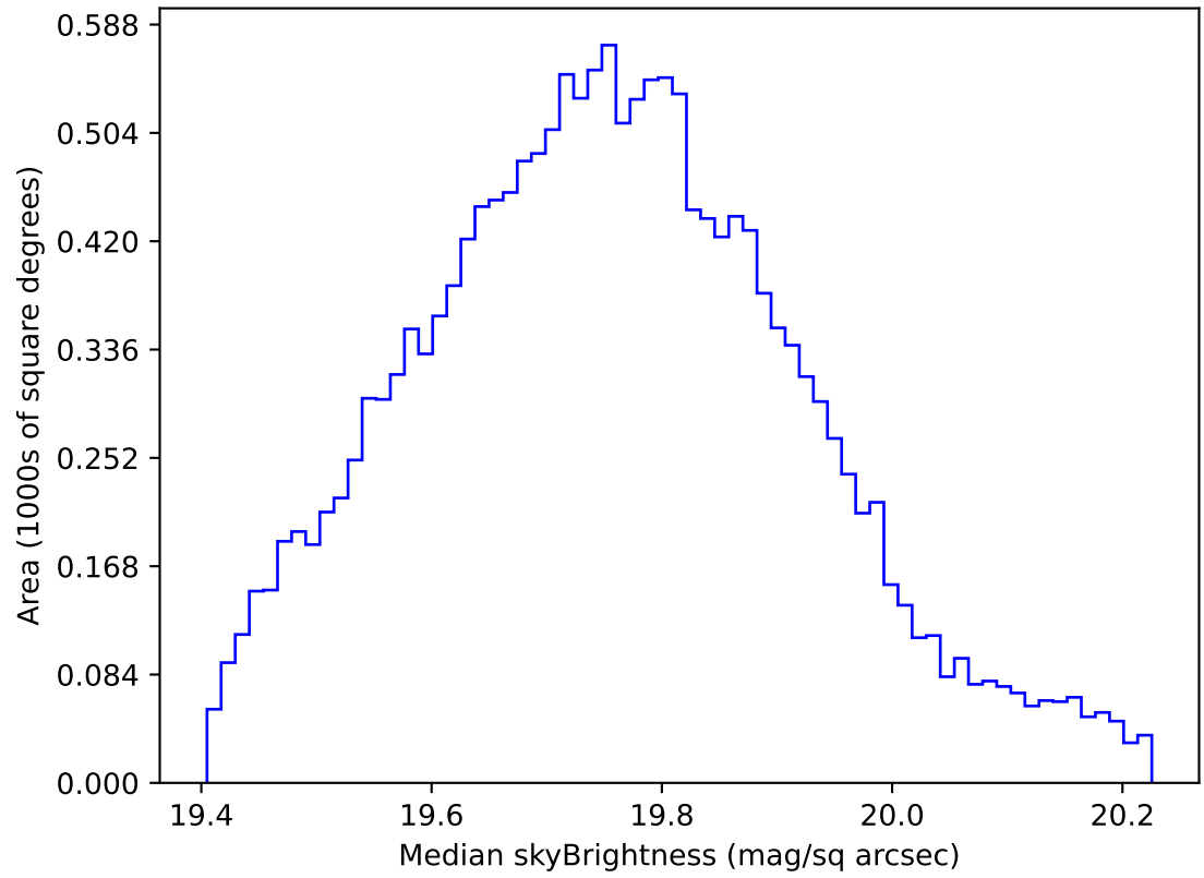
internal_u_expt27_nscale0.9v3.4_10yrs WFD all bands: Median skyBrightness
