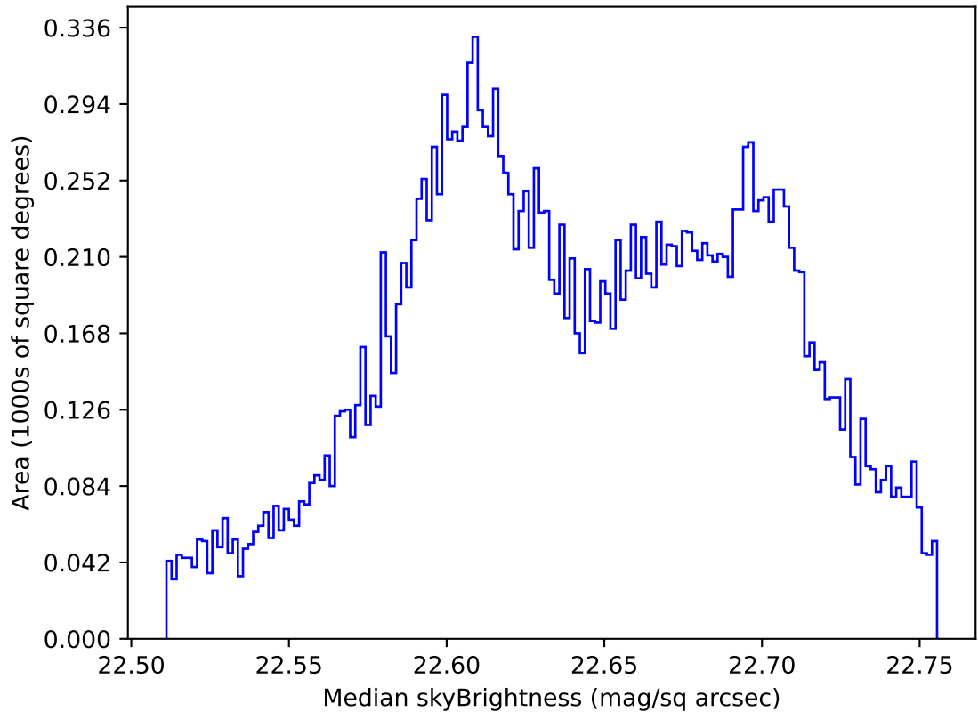
internal_u_expt27_nscale0.9v3.4_10yrs All sky u band: Median skyBrightness
