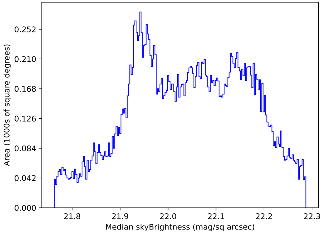
internal_u_expt27_nscale0.9v3.4_10yrs All sky g band: Median skyBrightness
