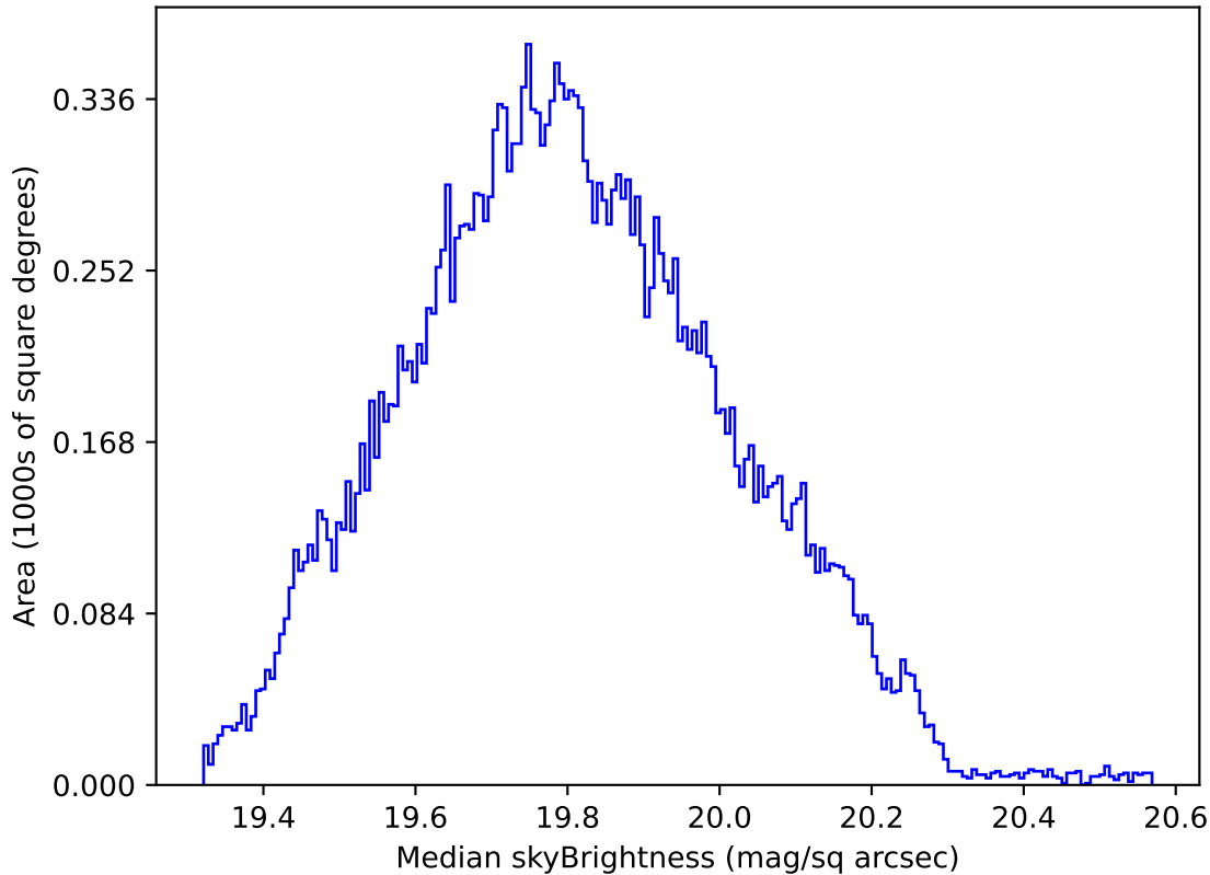
internal_u_expt27_nscale0.9v3.4_10yrs All sky all bands: Median skyBrightness
