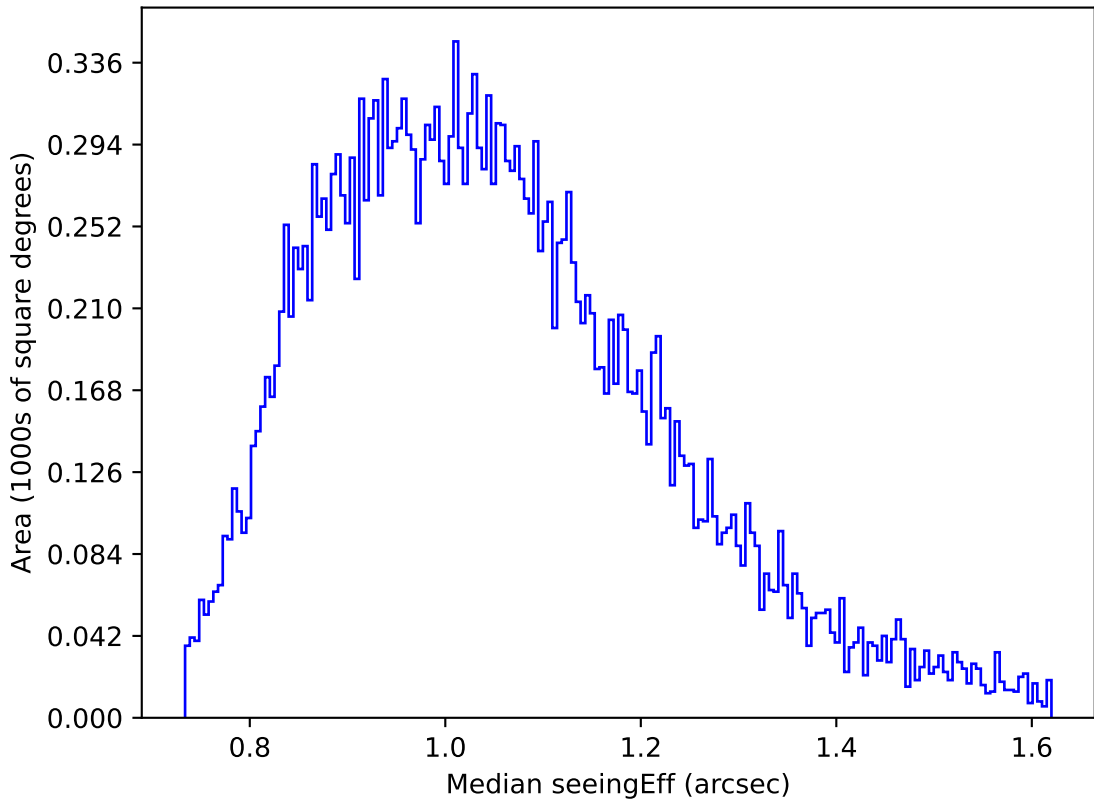
internal_u_expt27_nscale0.9v3.4_10yrs Yr 1 g band: Median seeingEff
