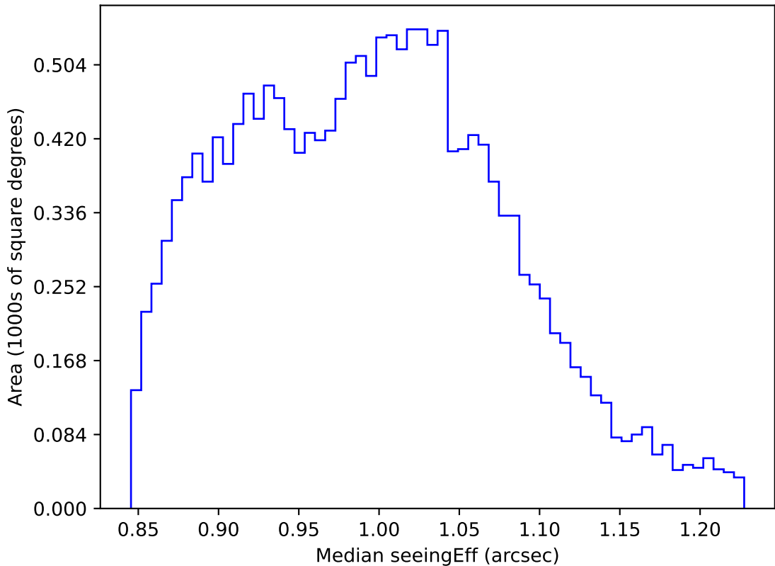
internal_u_expt27_nscale0.9v3.4_10yrs WFD i band: Median seeingEff
