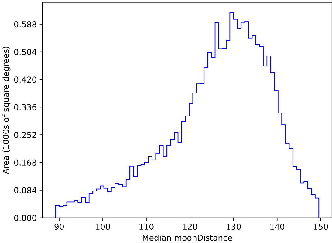
internal_u_expt27_nscale0.9v3.4_10yrs WFD u band: Median moonDistance
