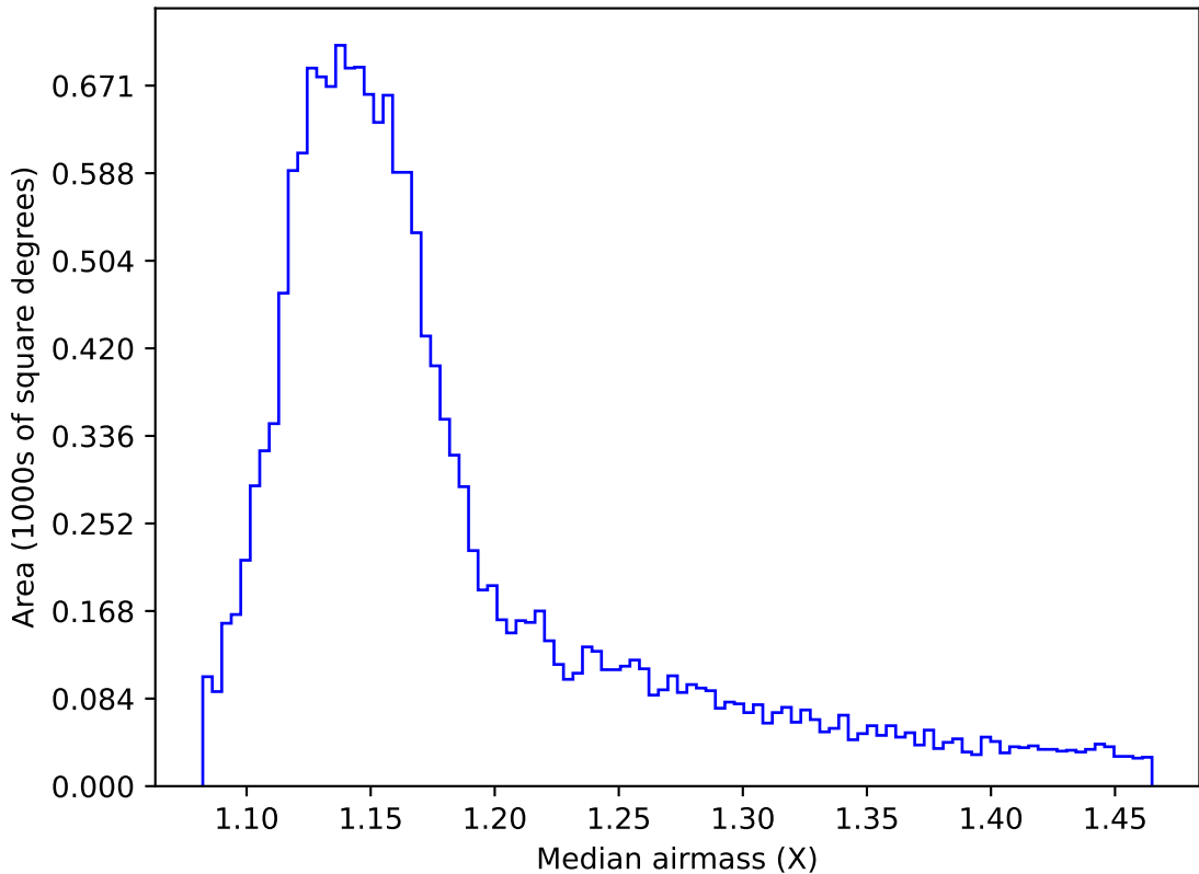
internal_u_expt27_nscale0.9v3.4_10yrs WFD z band: Median airmass
