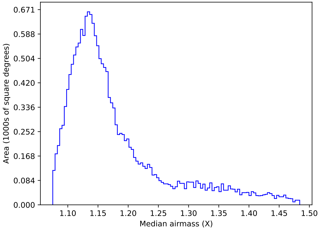
internal_u_expt27_nscale0.9v3.4_10yrs WFD g band: Median airmass
