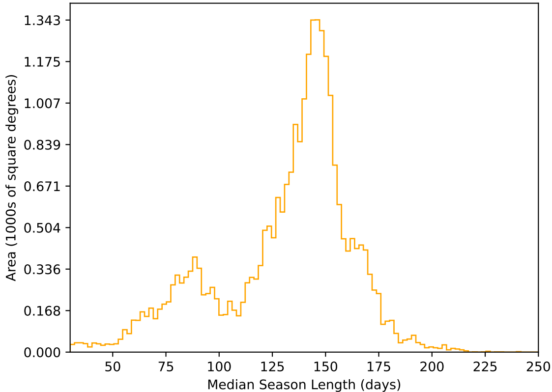
internal_u_expt27_nscale0.9v3.4_10yrs All sky r band: Median Season Length
