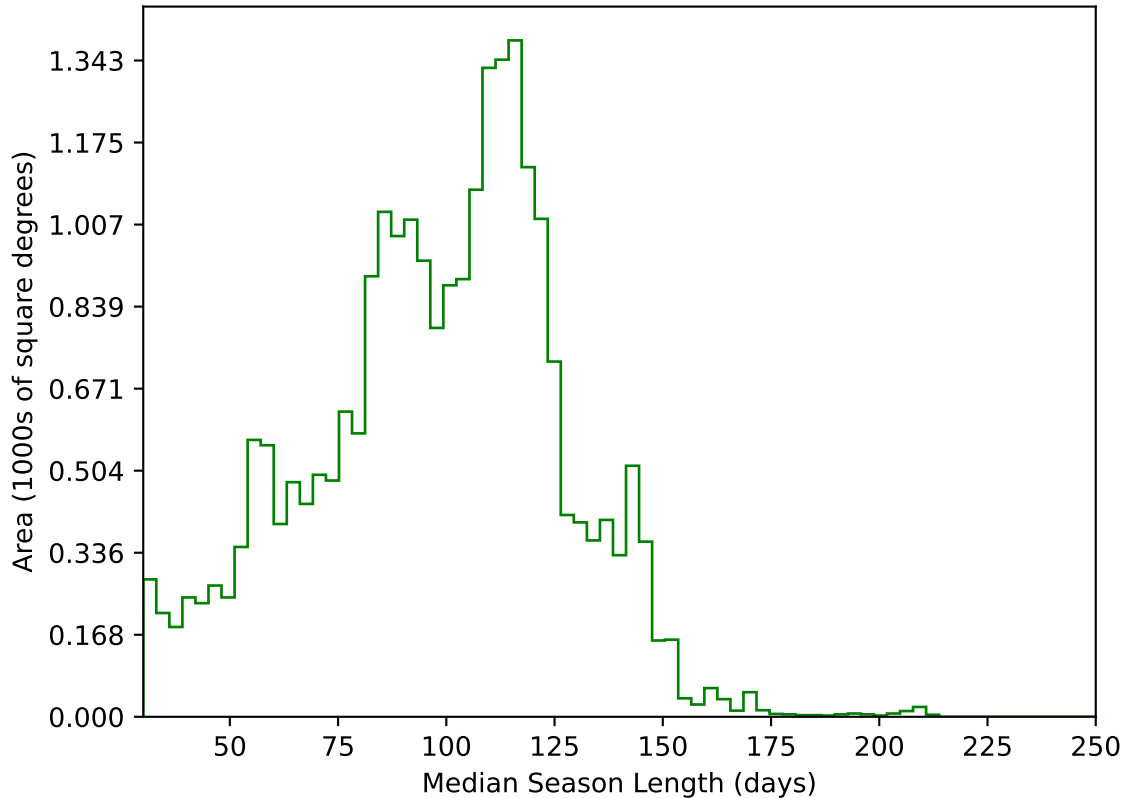
internal_u_expt27_nscale0.9v3.4_10yrs All sky g band: Median Season Length
