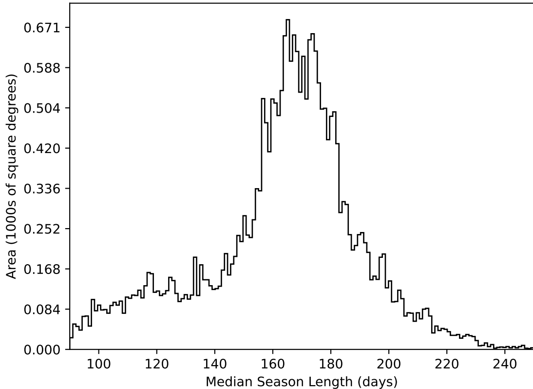
internal_u_expt27_nscale0.9v3.4_10yrs All sky all bands: Median Season Length
