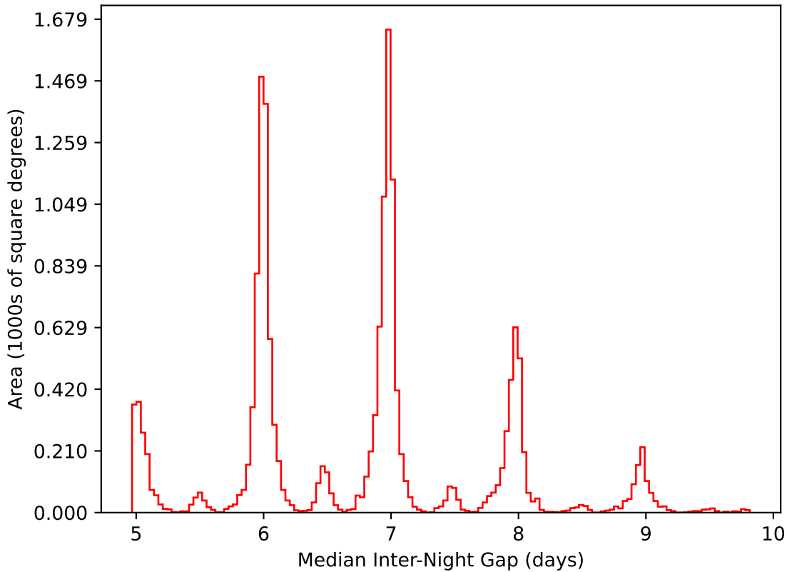
internal_u_expt27_nscale0.9v3.4_10yrs WFD i band: Median Inter-Night Gap
