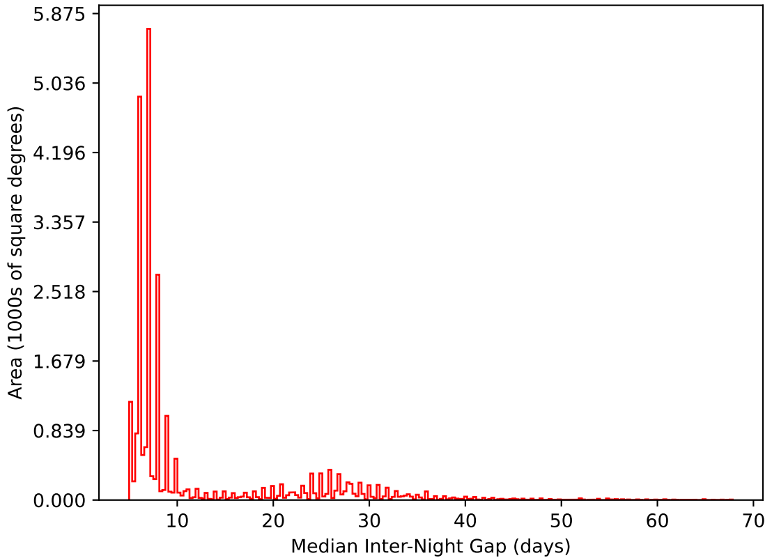
internal_u_expt27_nscale0.9v3.4_10yrs All sky i band: Median Inter-Night Gap
