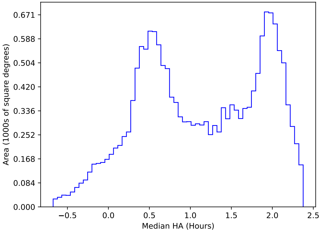
internal_u_expt27_nscale0.9v3.4_10yrs WFD z band: Median HA
