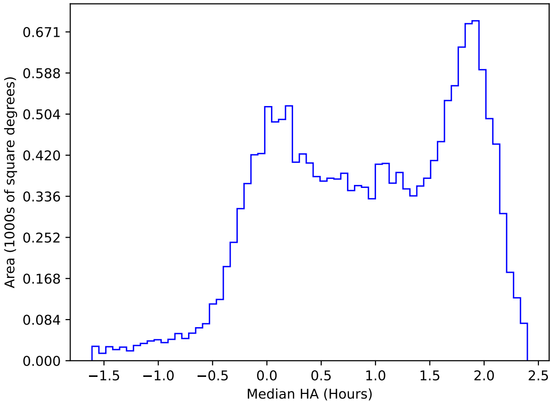
internal_u_expt27_nscale0.9v3.4_10yrs WFD u band: Median HA
