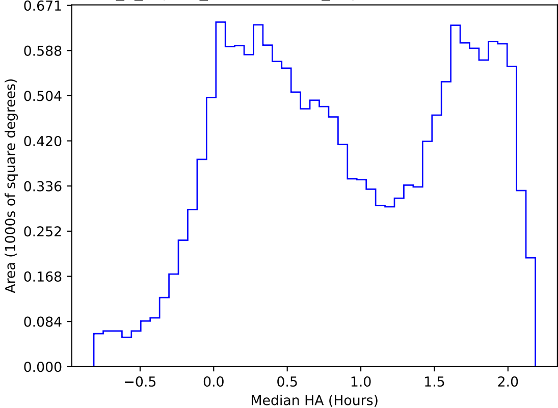
internal_u_expt27_nscale0.9v3.4_10yrs WFD r band: Median HA
